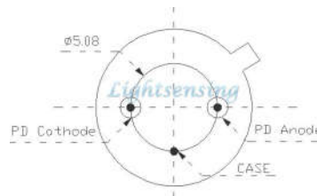
3PIN Bottom View
